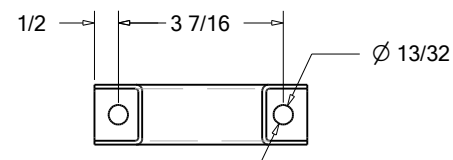
Caster Mount Tube 1-1/4 x 1-1/4 x .083 wall steel tube 8 pcs
