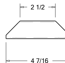
Caster Mount Tube 1-1/4 x 1-1/4 x .083 wall steel tube 8 pcs
