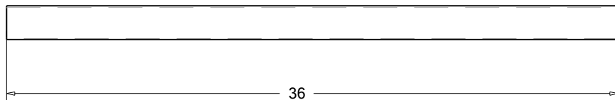
Front Top Cross Tube 2 x 2 x .083 wall steel tube
